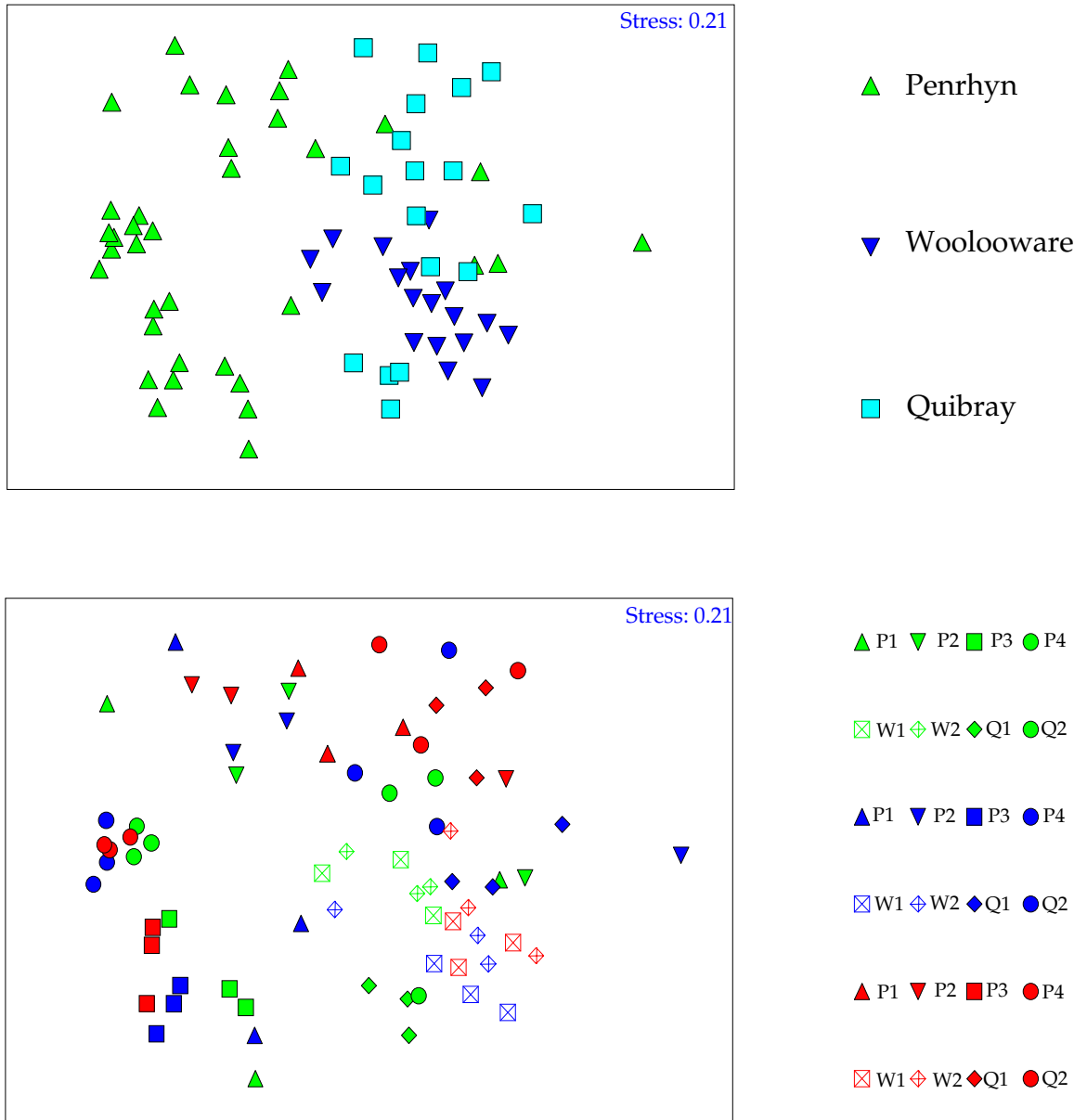
Figure 6: MDS ordinations comparing saltmarsh assemblages across (a) locations and (b) sites and times (P = Penrhyn Estuary, W = Woollooware Bay, Q = Quibray Bay, 1-4 = Sites, Green = Survey 1, Blue = Survey 2 and Red = Survey 3).
