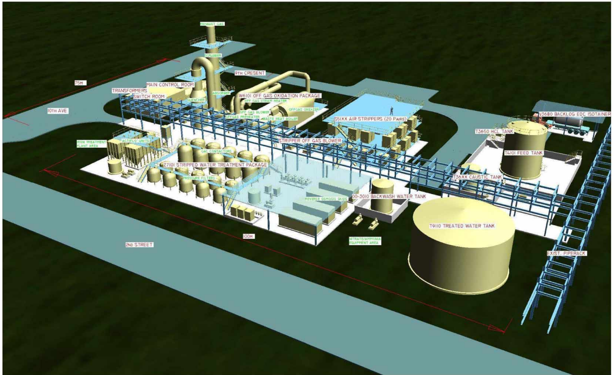
FIGURE ES-3 Groundwater Treatment Plant Visual Simulation
