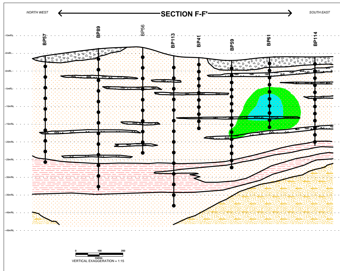
CARBON TETRACHLORIDE
