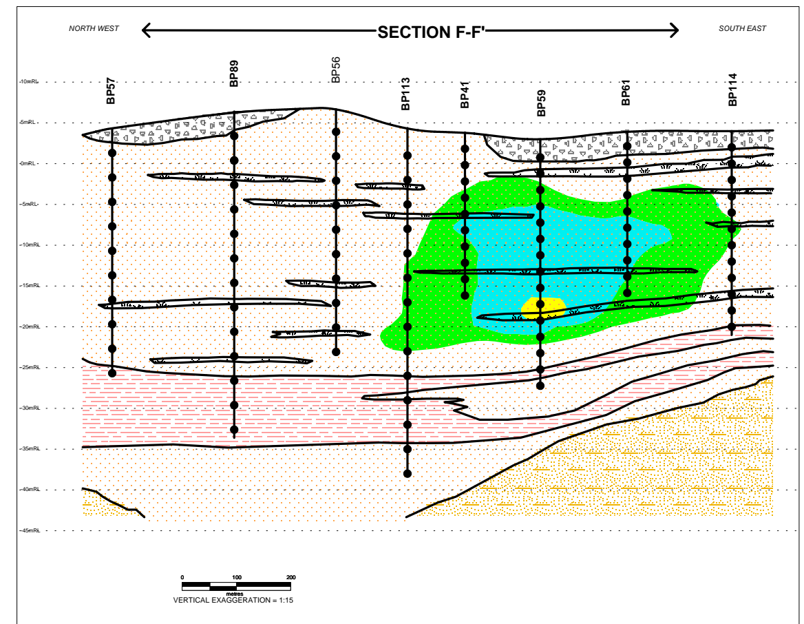
1,1,2-TETRACHLOROETHANE
