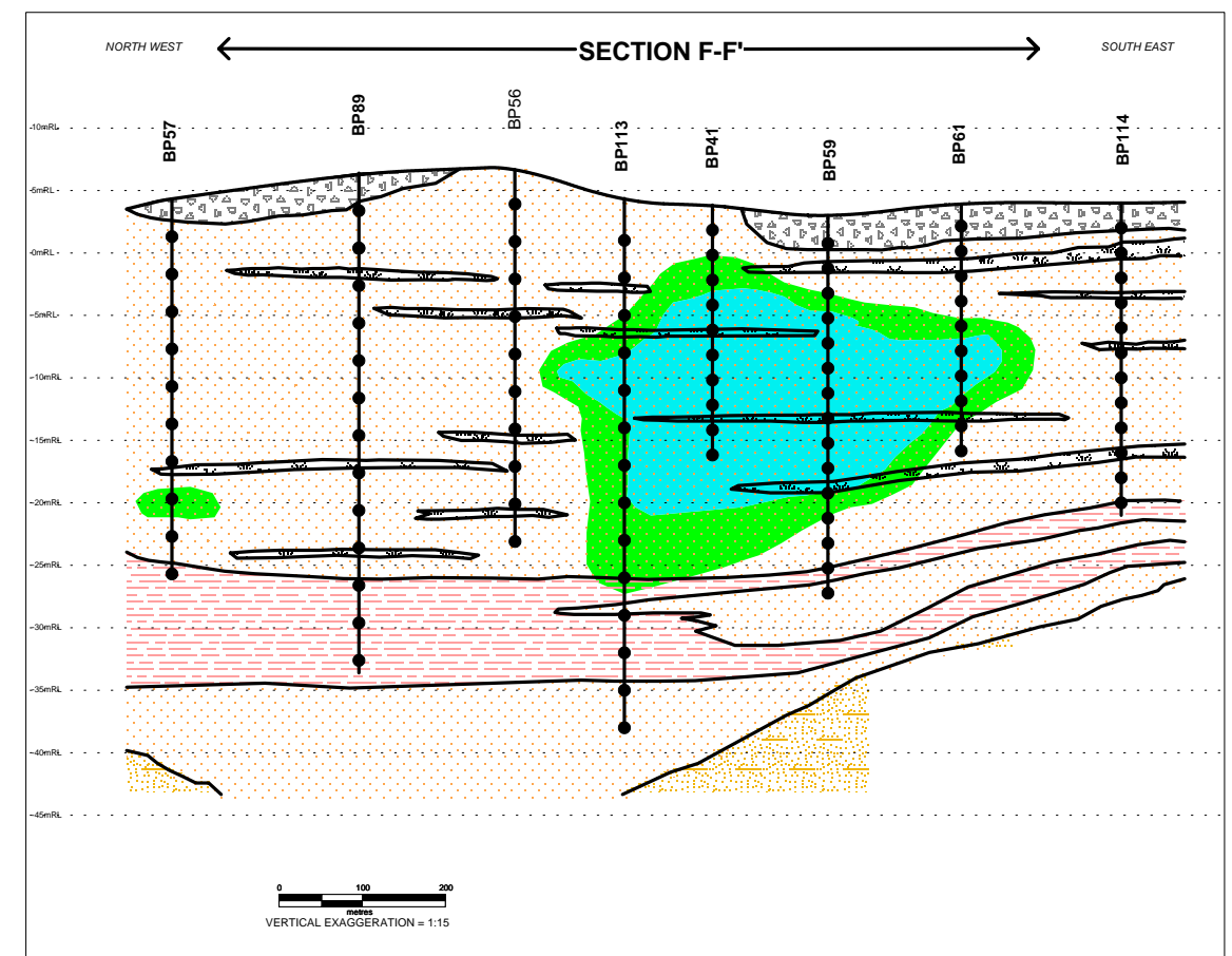
1,1,2-TRICHLOROETHANE
