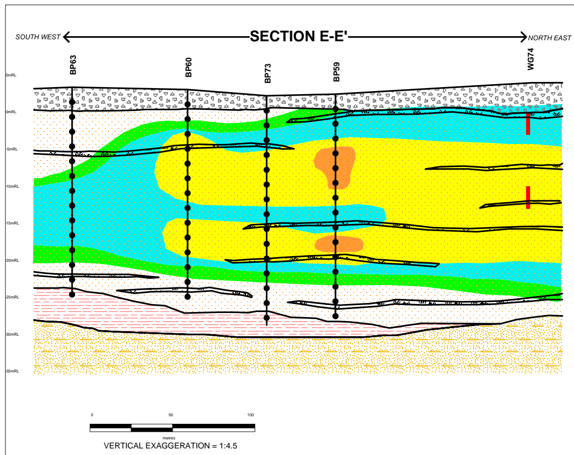
VINYL CHLORIDE
