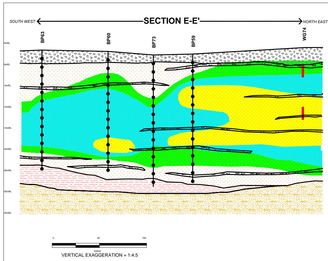
TRICHLOROETHENE
