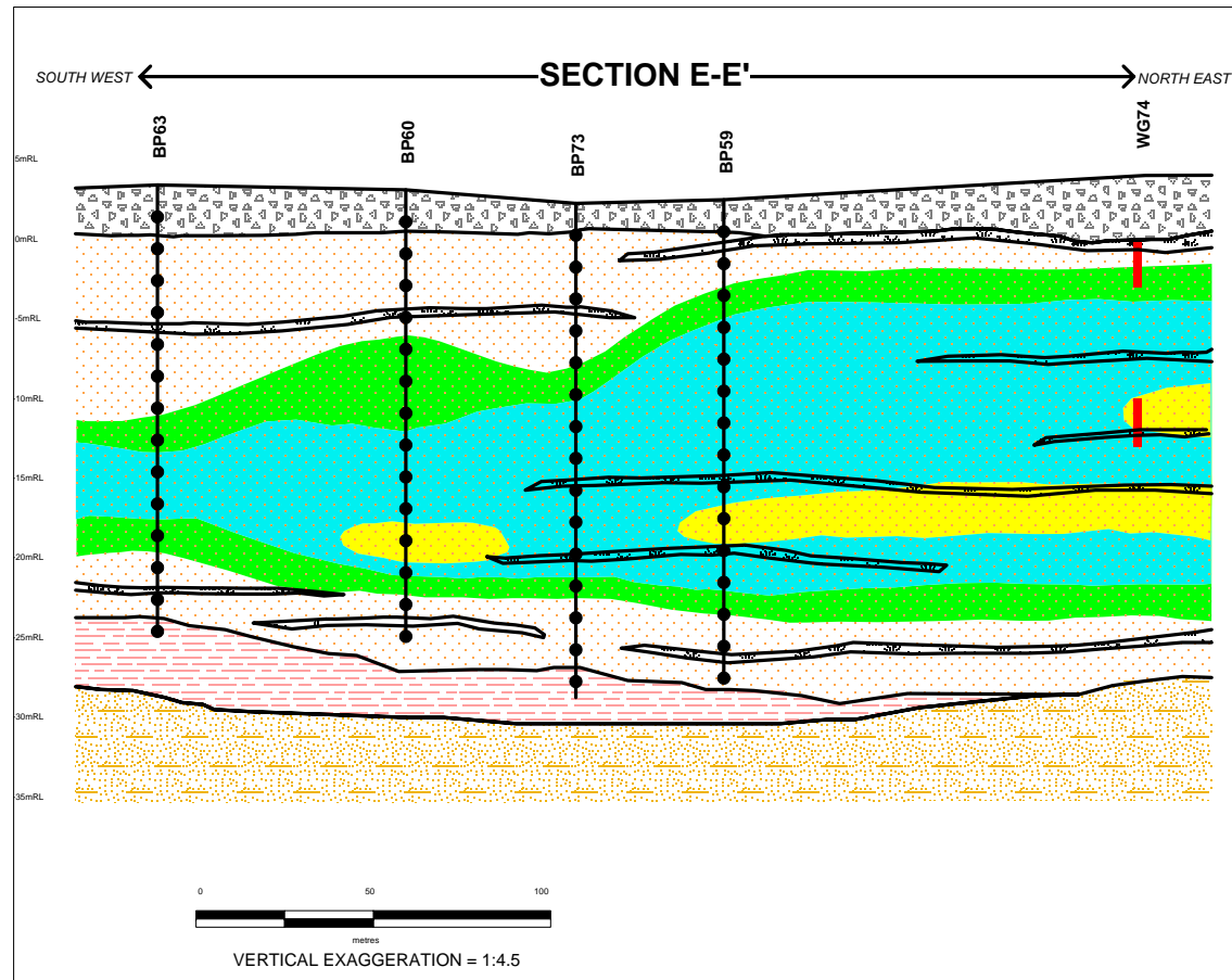
TETRACHLOROETHENE
