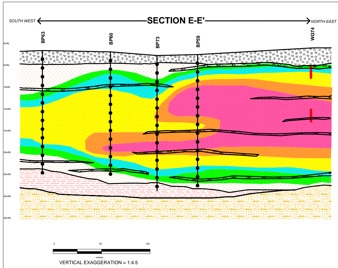
1,2-DICHLOROETHANE
