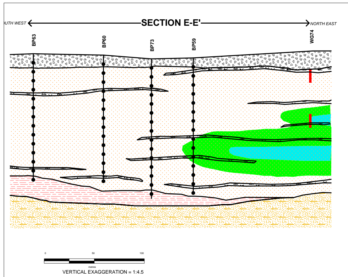
CARBON TETRACHLORIDE
