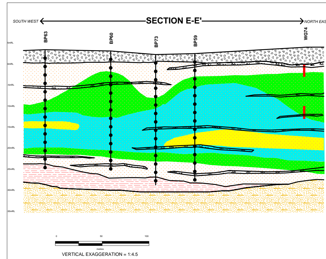
1,1,2,2-TETRACHLOROETHANE
