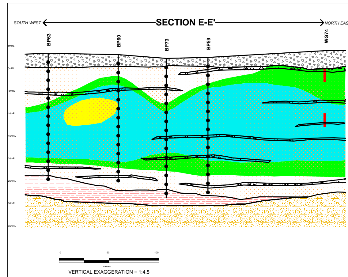
1,1,2-TRICHLOROETHANE
